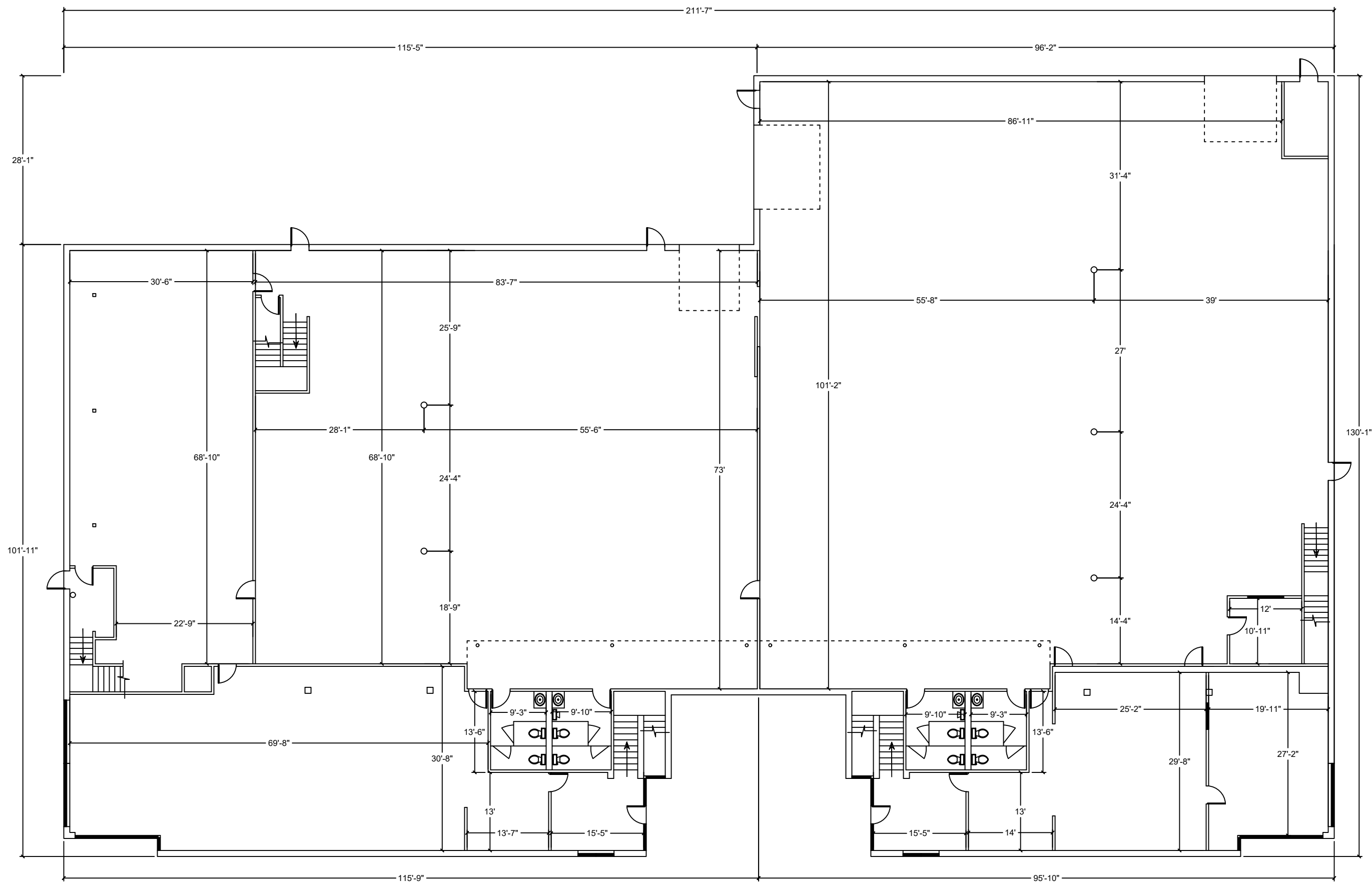
2 Stage 14 Floor Plan (Dimension) A3 Total 1st Floor Sq. Ft - 11,300 • Stage - 6,040 • Office - 5,260
