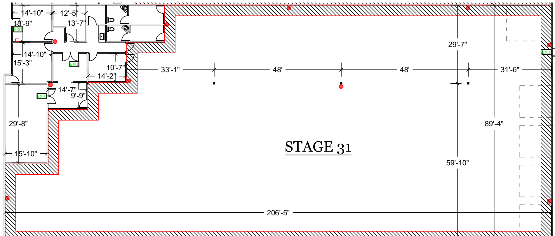
3 First Floor Plan - Stage 31 A4 Office Sq. Ft - 2,170 Stage Sq. Ft. - 16,300
