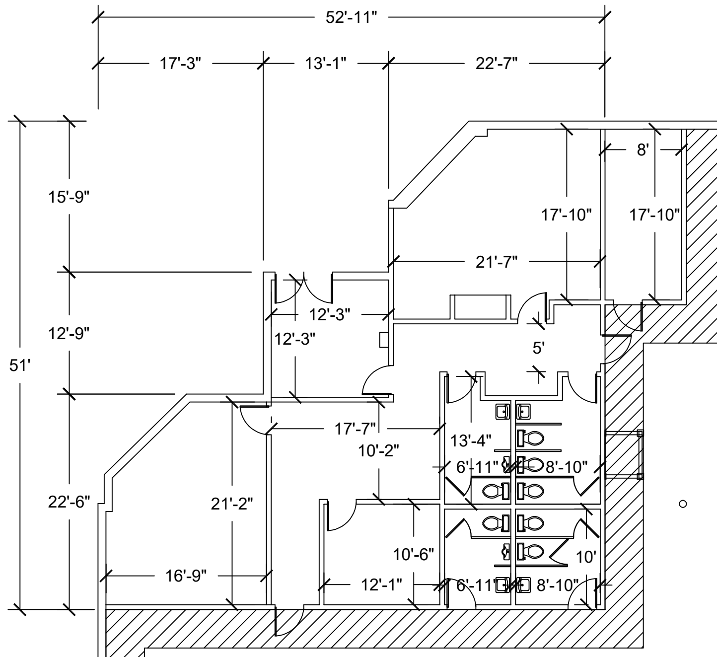
2 Overall Plan - Office A2 Dimension
