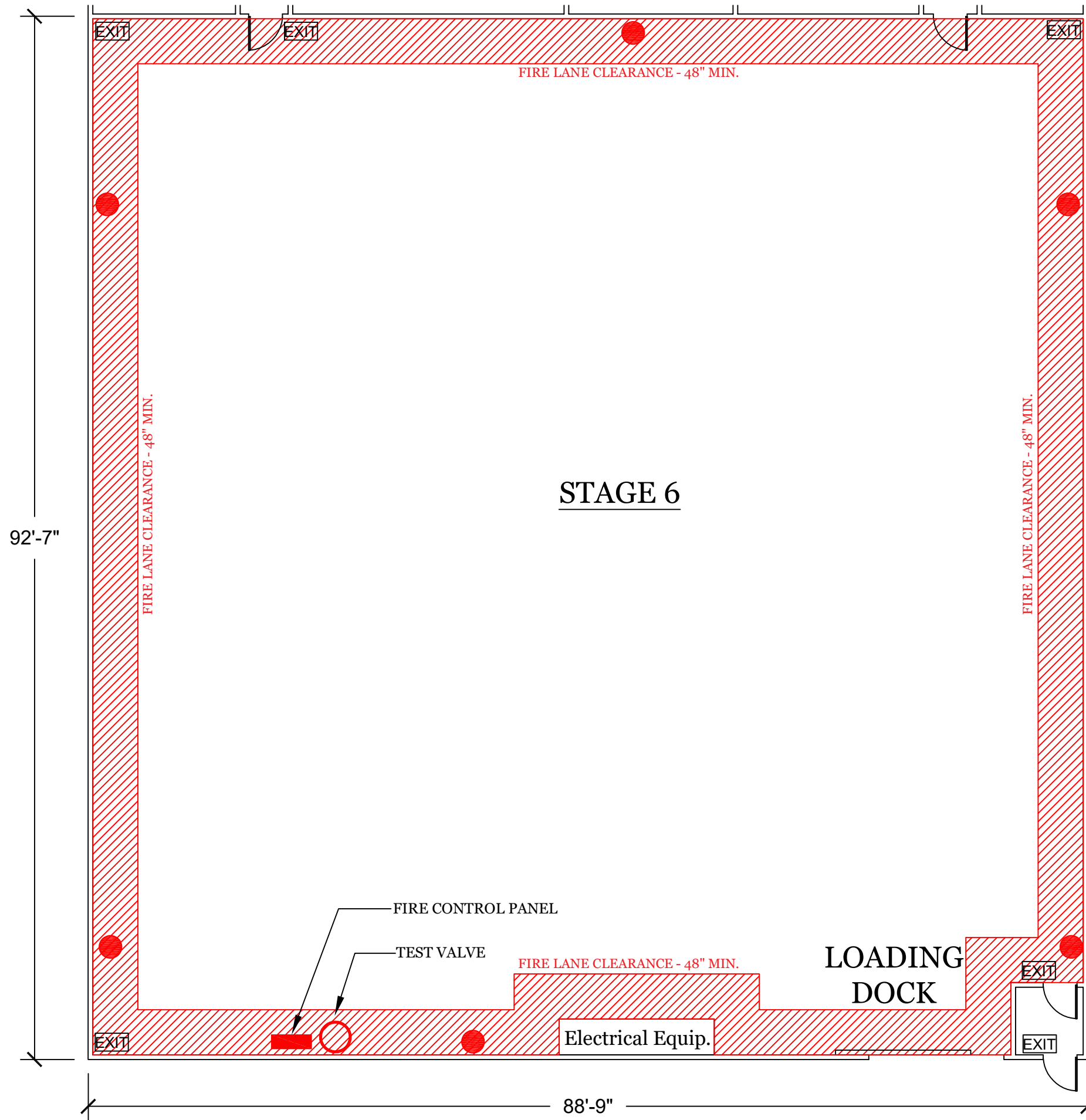
1 Stage 6 Floor Plan A3 Sq. Ft - 8,225
